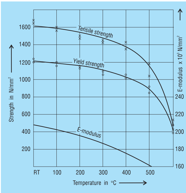
Figure 38 Yield stress and 'E' modulus of steel X 22 CrMoV 12 1 with respect to temperature.
