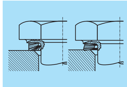
Figure 42 Bolt with SCHNORR Safety Washer loose and tightened
