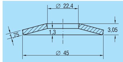
Figure 11 Disc spring 45 x 22.4 x 1.75; l_0 = 3.05 mm
