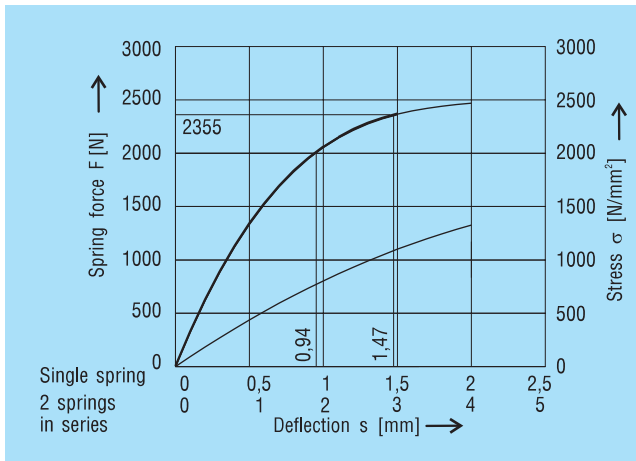
Figure 14 Diagram for spring 60 x 30.5 x 1.5 mm, l_0 = 3.5 mm
