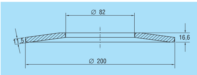
Figure 15 Disc spring 200 x 82 x 12 mm
