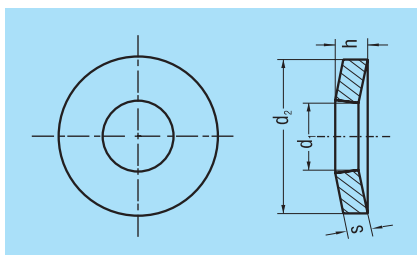
Figure 45 HDS Load Washer
