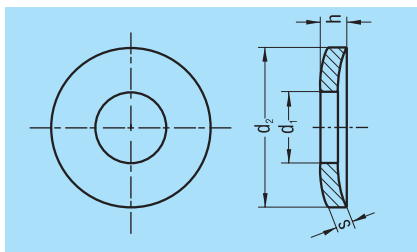
Figure 46 Original SCHNORR High Load Safety Washer “HS”
