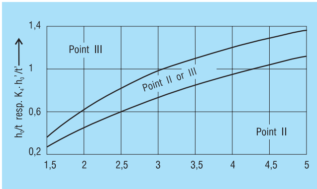
Figure 17 Decisive point of cross-section to be used to determine fatigue life
