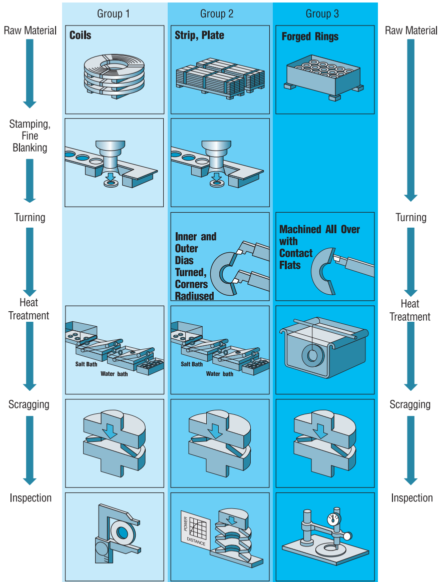
Figure 27 The manufacturing process of several groups
