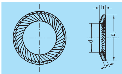
Figure 43 Original SCHNORR Safety Washer type “S”
