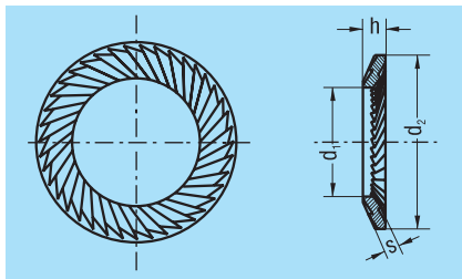
Figure 44 Original SCHNORR Safety Washer type „VS“
