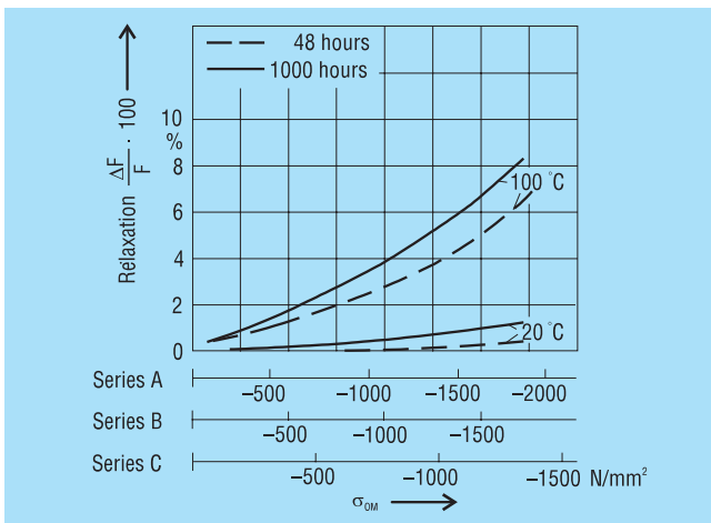
Figure 30 Permissible relaxation for disc springs of chrome and chrome- vanadium-alloy steel as per DIN 17 221 and DIN 17 222.
